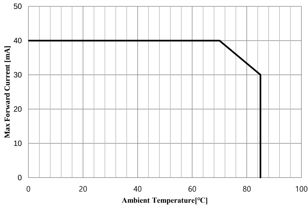
FIG 8. Max. Forward current vs Ambient Temperature (RthJ-B : 20°C/W)
