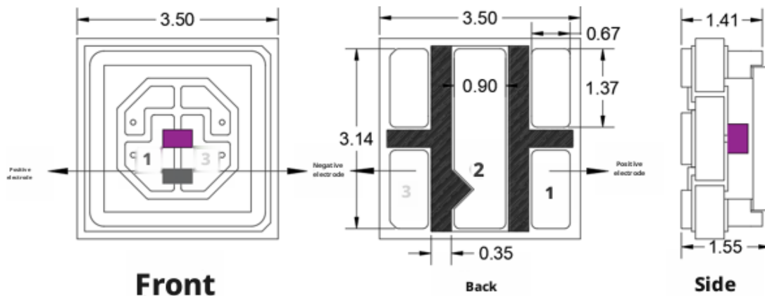
Device Dimensions
