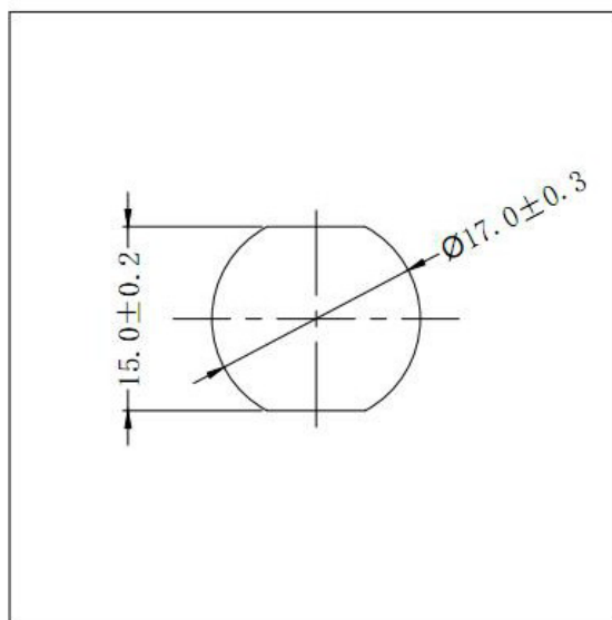
Cutout Size
