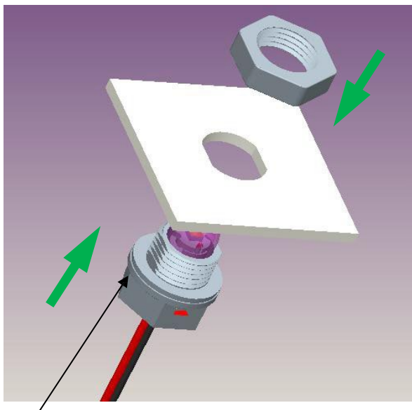
Waterproof Gasket
