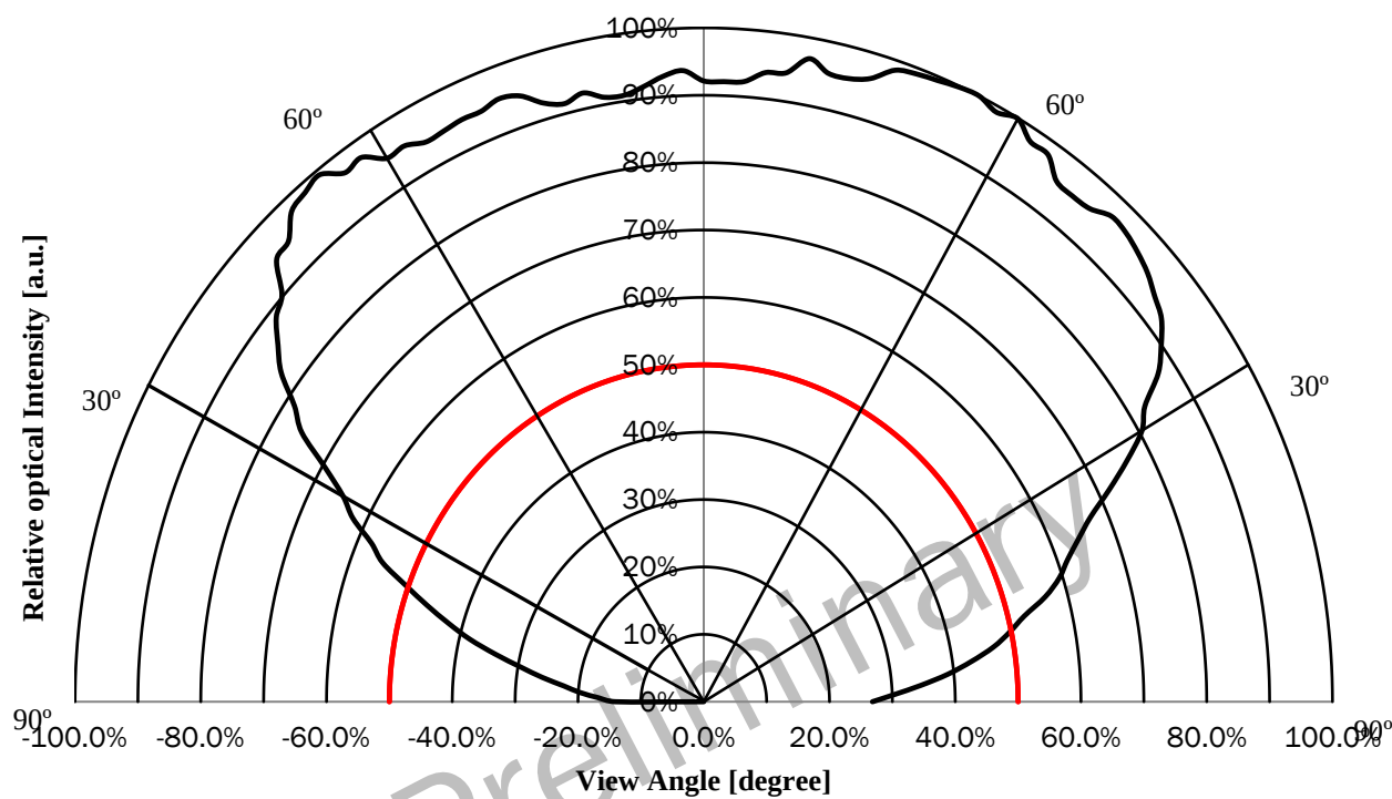
FIG 7. Far-field Emission Pattern
